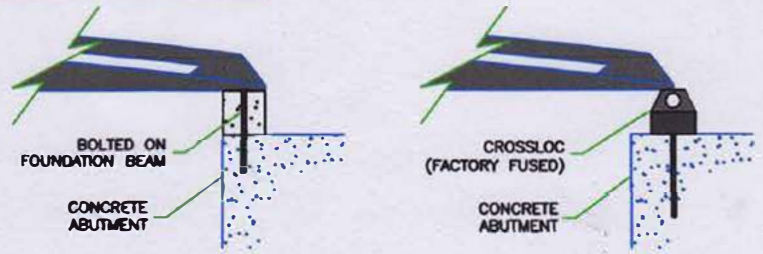
TYPICAL INSTALLATION
